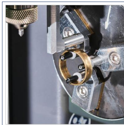
Ring Roll-off Engraving
